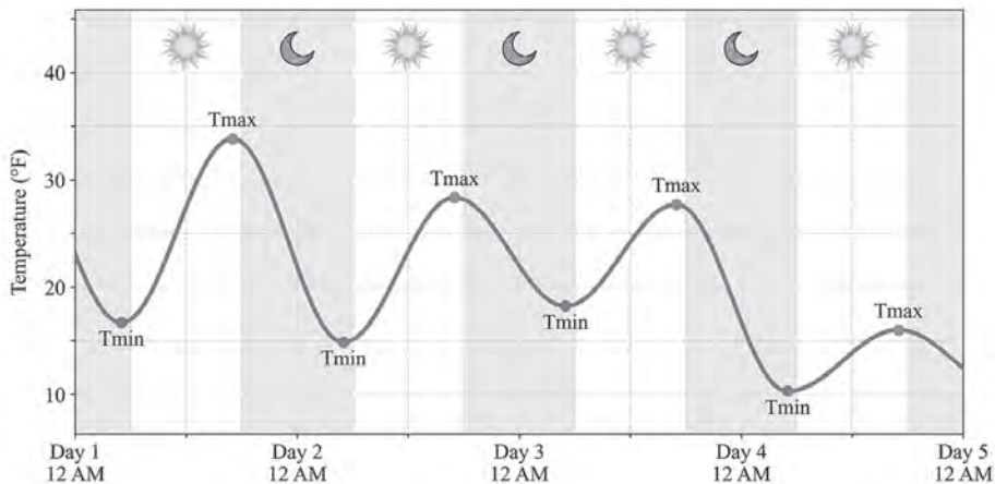
Figure 1.1. Graph of typical diurnal variations of temperature, where Tmax is an example of a daily maximum and Tmin is a daily minimum. Note that this general pattern can vary with geographic location and changing weather conditions.
